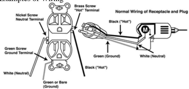
Correct Wiring
